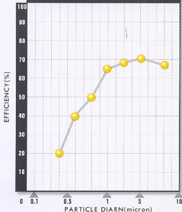
EFFICIENCY VS. PARTICLE DIARN
